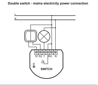
Fig.1 Wiring diagrams for Fibaro Switch.
