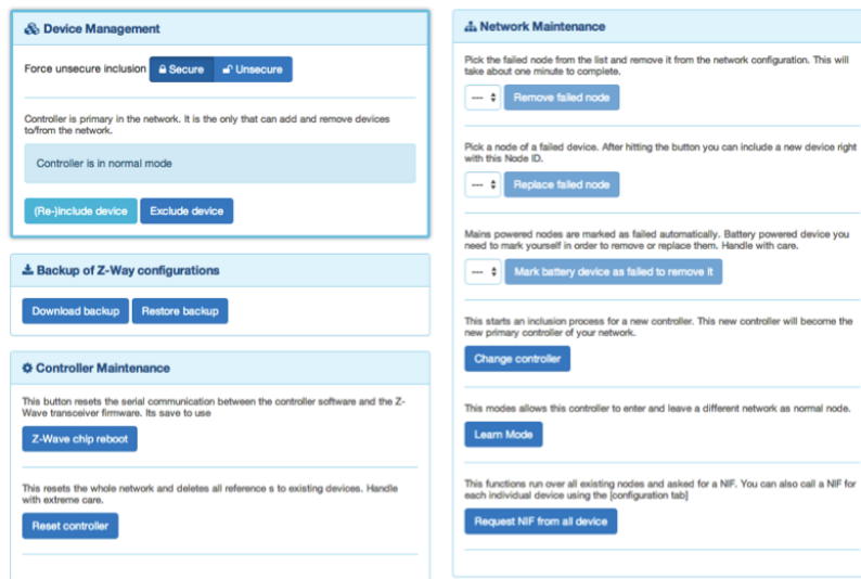
Figure 2.6: Expert UI Dialog for Networking functions
