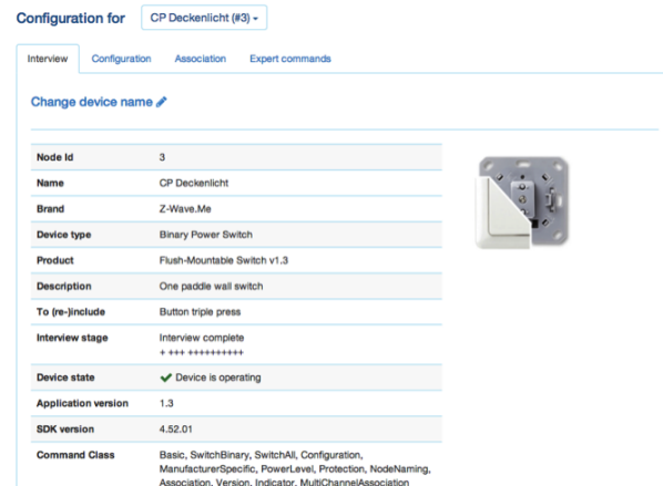
Figure 2.10: Configuration Dialog
